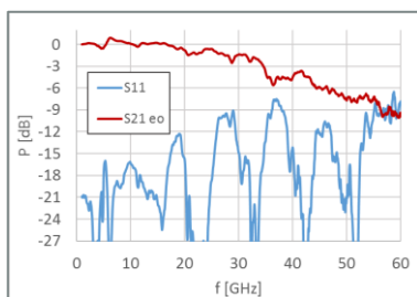
Small signal response
